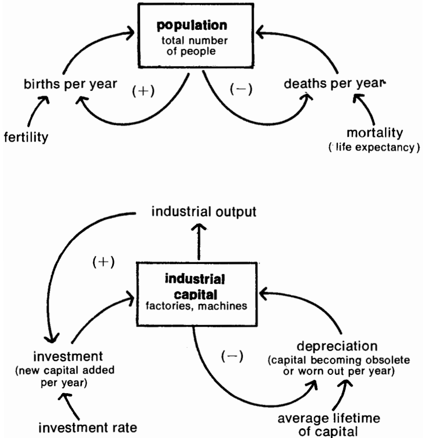
Figure 23 POPULATION GROWTH AND CAPITAL GROWTH FEEDBACK LOOPS
