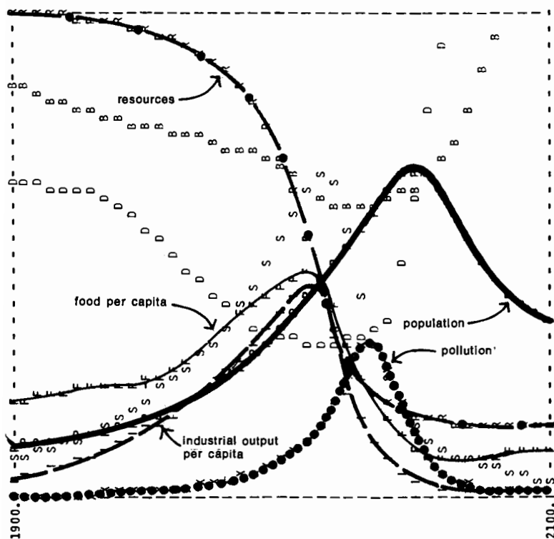
Figure 35 WORLD MODEL STANDARD RUN
