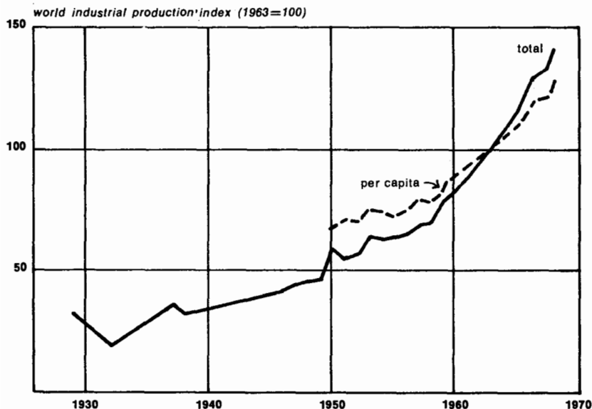
Figure 6 WORLD INDUSTRIAL PRODUCTION
