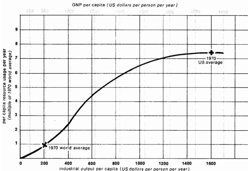
Figure 28 INDUSTRIAL OUTPUT PER CAPITA AND RESOURCE USAGE
