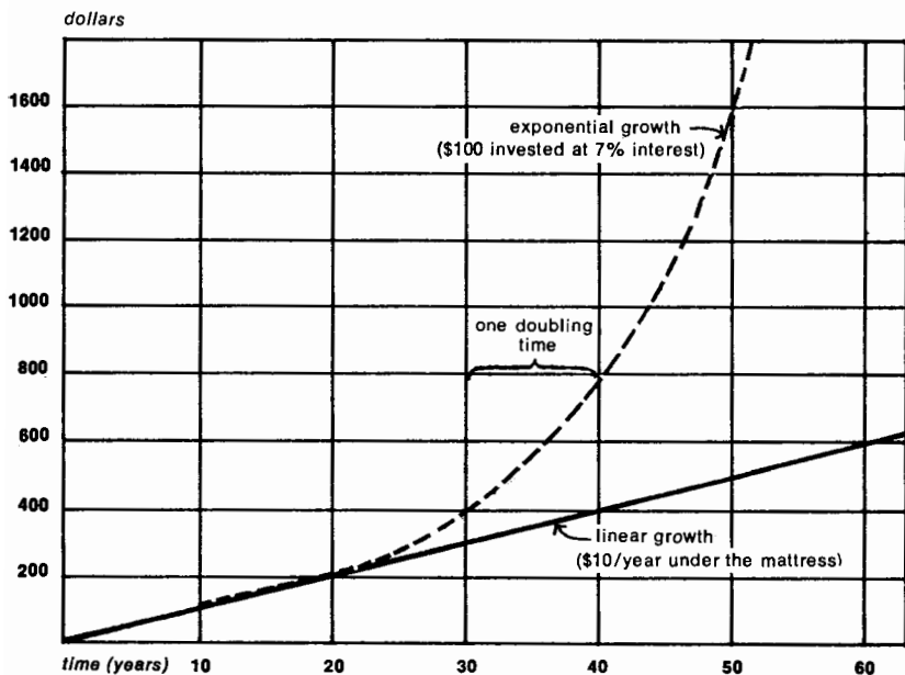
Figure 4 THE GROWTH OF SAVINGS
