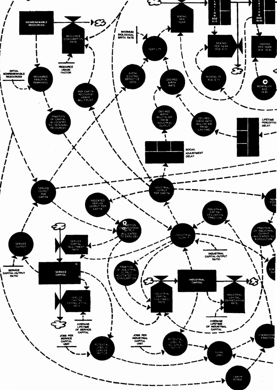
Figure 26 THE WORLD MODEL
