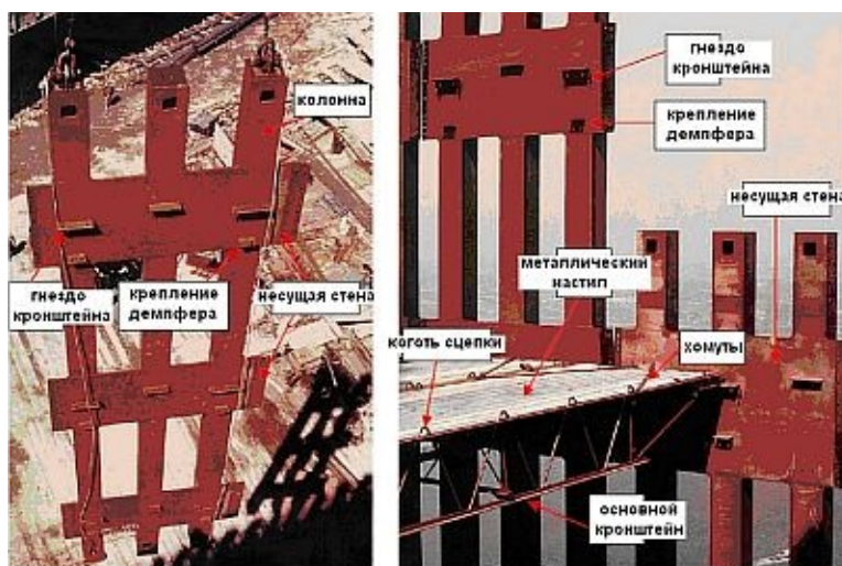
Figure 1–4. Perimeter column/spandrel assembly and floor structure.
